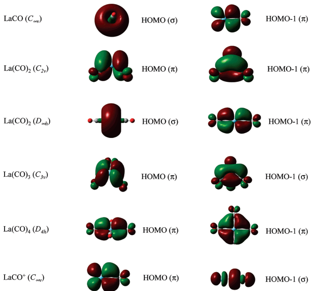
Figure 7. Molecular orbital depictions of the highest occupied molecular orbitals (HOMOs) and HOMO-1s of the La(CO) n ( n = 1–4) and LaCO + molecules
